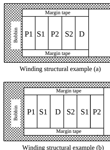
Figure 10-4 Winding structural examples
